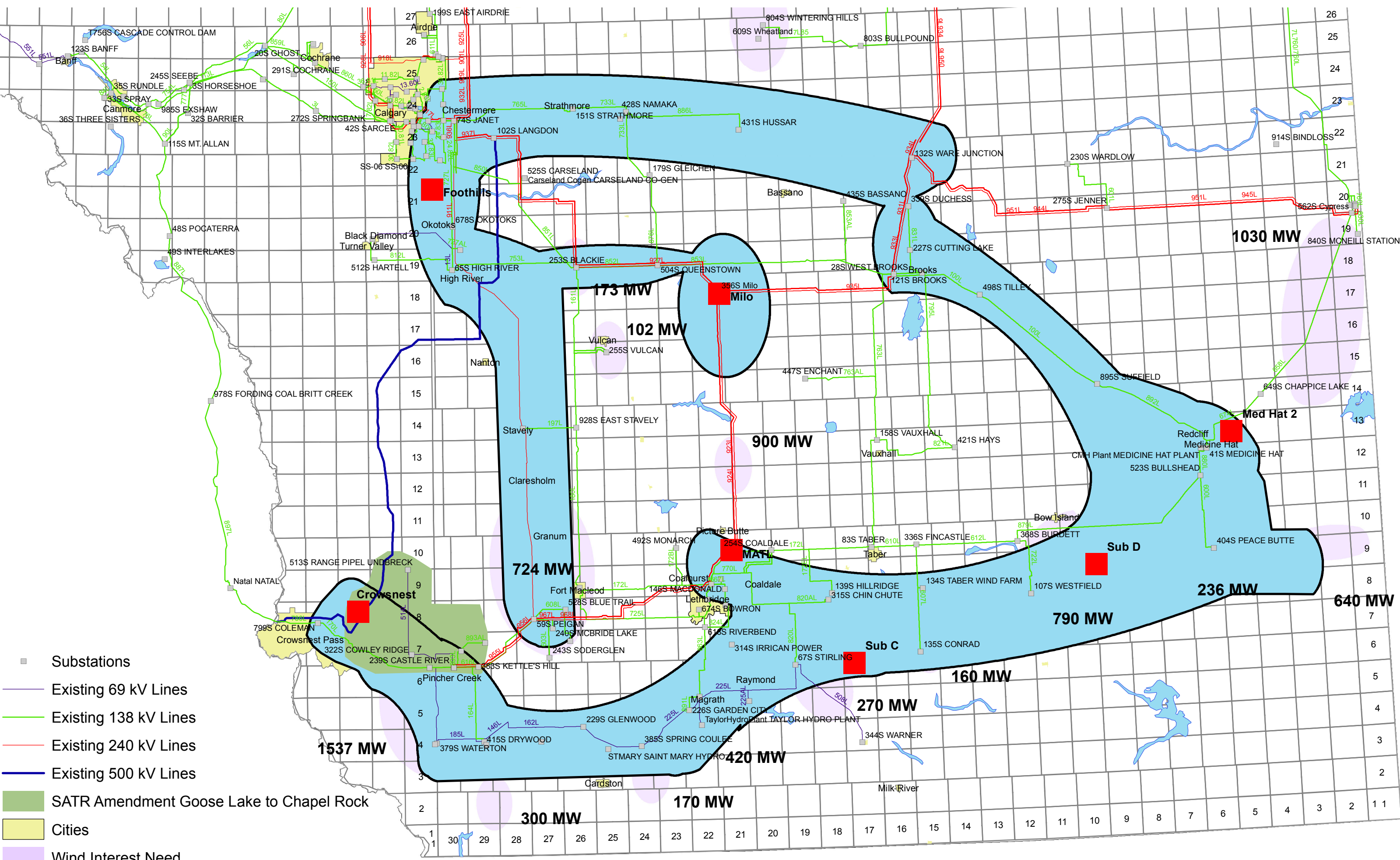
240 kV Alternative - Looped System 1A
